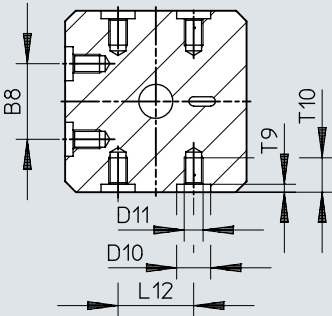
Dimensions – Swivel/gripper units HGDS-12 – cut at [1]
