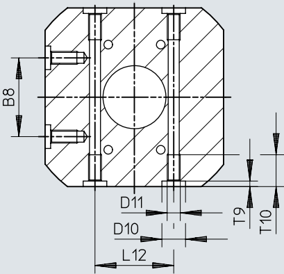
Dimensions – Swivel/gripper units HGDS-20 – cut at [1]
