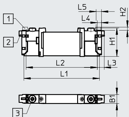
[1] Vertical electrical connection [2] Horizontal electrical connection [3] Manual override
