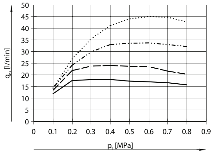
Suction volume flow q_{nS} as a function of working pressure p_1
