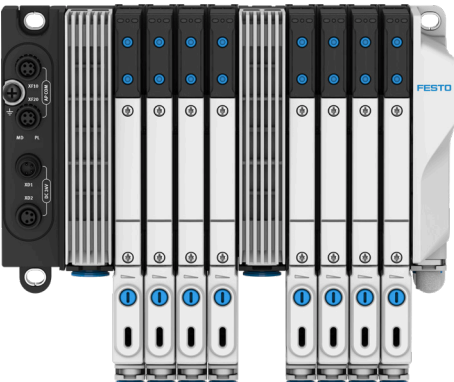
8 manifold sub-bases with intermediate supply
