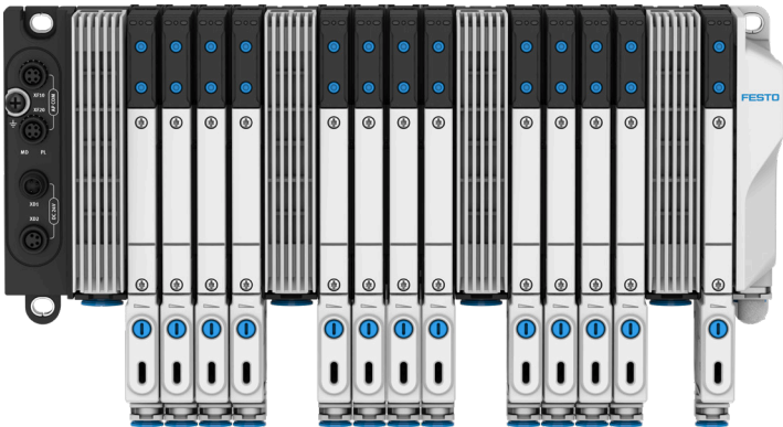
13 manifold sub-base with intermediate supply
