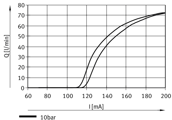
Characteristic flow rate curve, nominal width 1.5 mm, 2 bar and 4 bar
