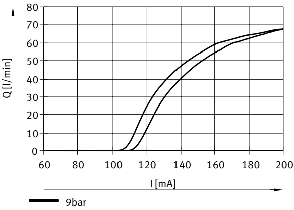
Characteristic flow rate curve, nominal width 1.5 mm, 1 bar and 3 bar
