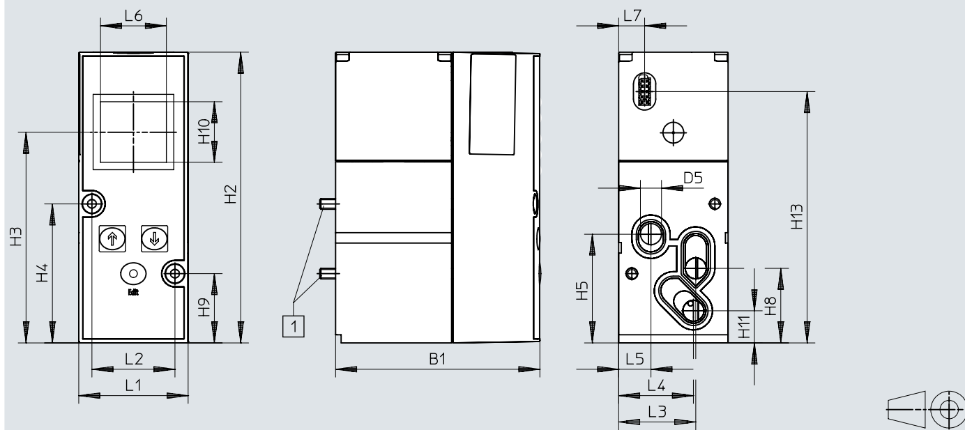
Dimensions – Analogue interface, VPPM-8TA, sub-base valve with LCD
