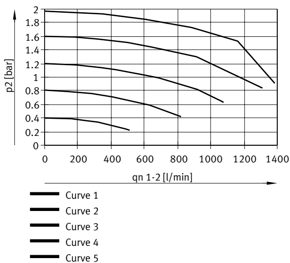
Flow rate q_{n1-2} from 1 -> 2 as a function of excess output pressure p_{2+} , VPPM-8F/8TA-...-0L2H-... (2 bar)
