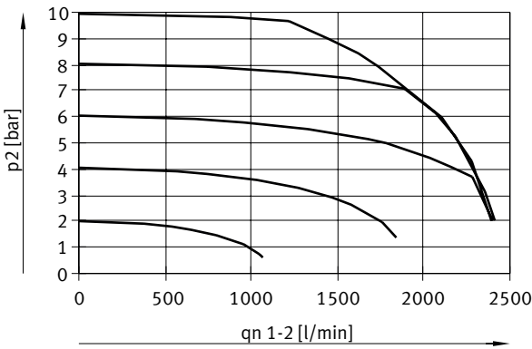
Flow rate qn from 1 -> 2 as a function of excess output pressure p2, VPPM-8F/8TA-...-0L10H-... (10 bar)
