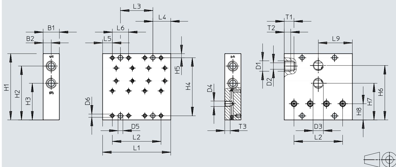
Dimensions – Manifold rail, connection direction underneath
