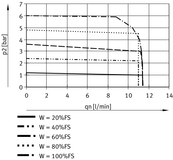
VEAA-...-D9-..., output pressure 2 (pressure regulation range) 0.03 ... 6, flow rate qn from 1 -> 2 depending on output pressure p2
