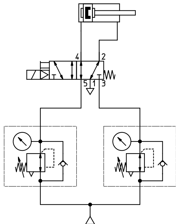
Dual-pressure operation with reversible regulator
