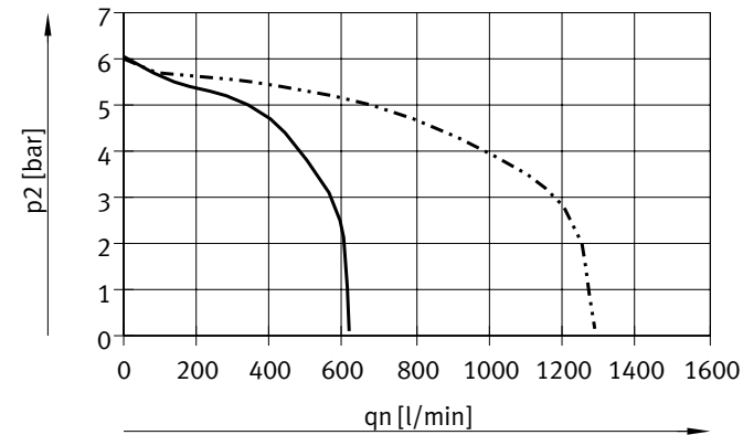
Flow rate q_n as a function of output pressure p_2 with pressure regulator plates (AB regulator plates, rev.) for ports 4/2, reversible 6 bar 10 bar
