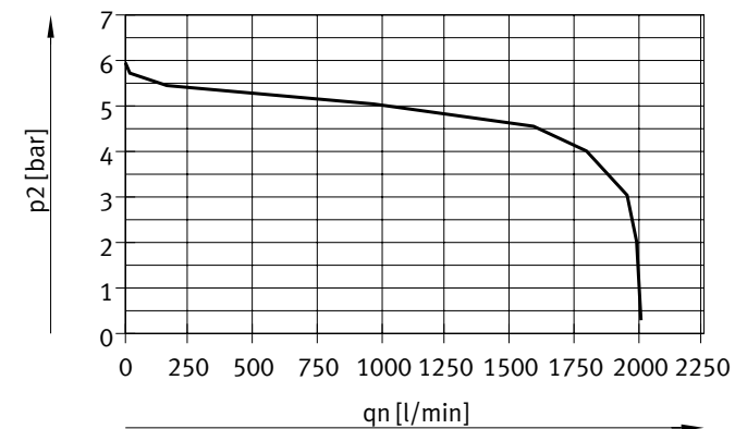
Input pressure 10 bar, regulated pressure set to 6 bar
