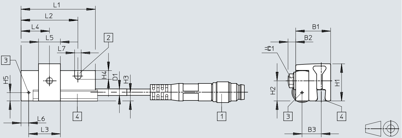
Dimensions – SMT-C1
