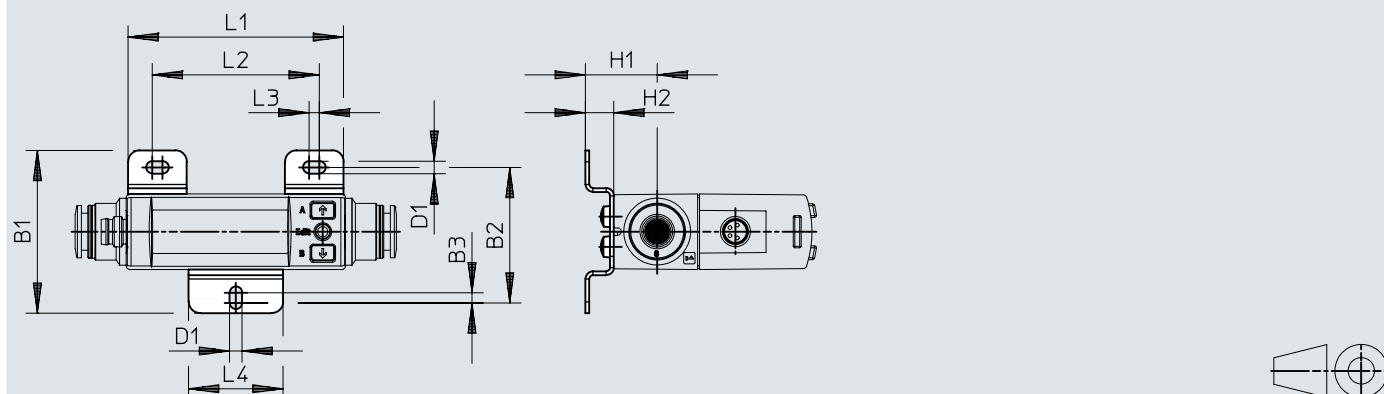
Dimensions – Wall mounting SAMH-FH-W
