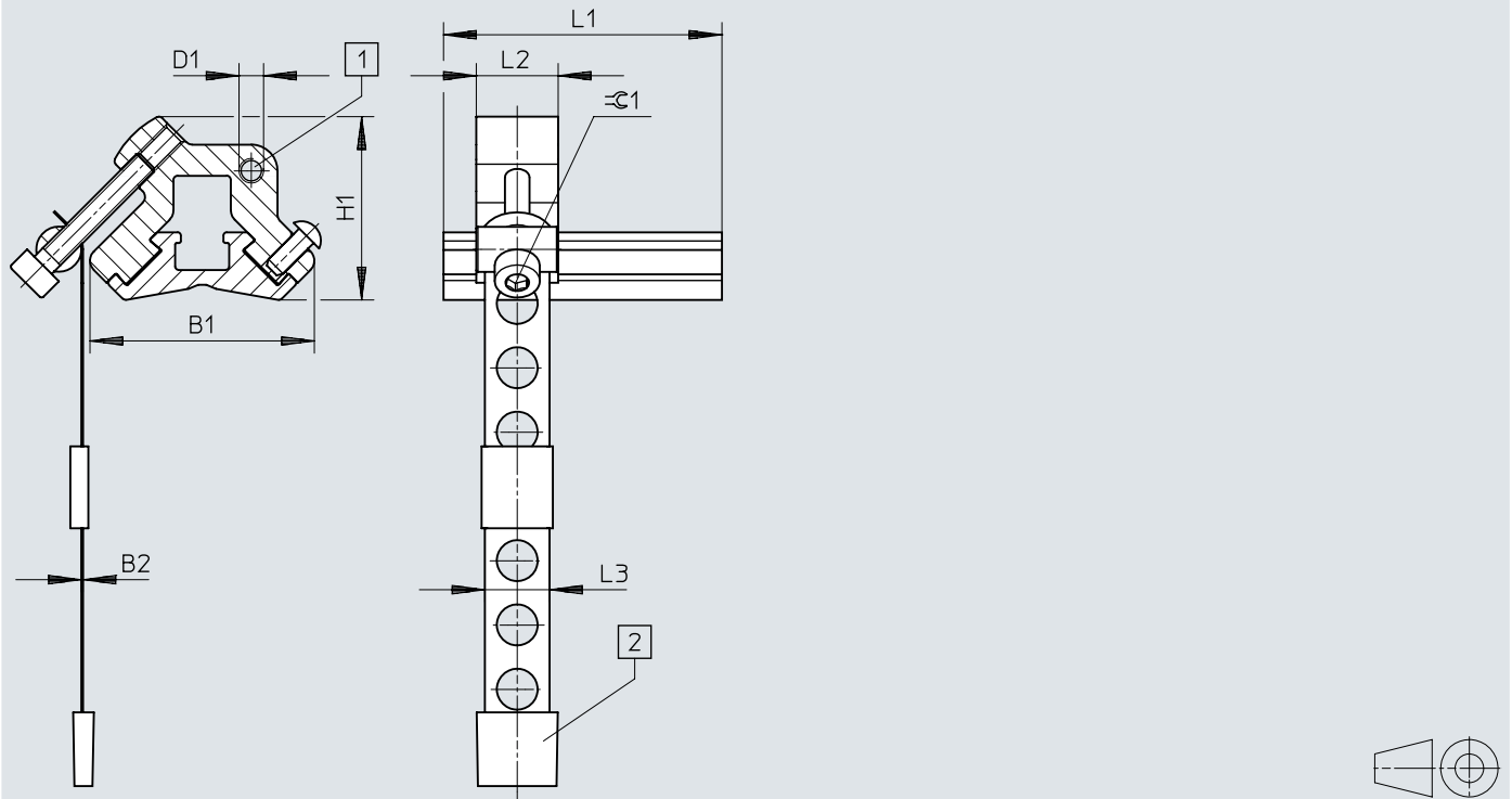
Dimensions – Mounting kit SMBR-8-8/100-S6
