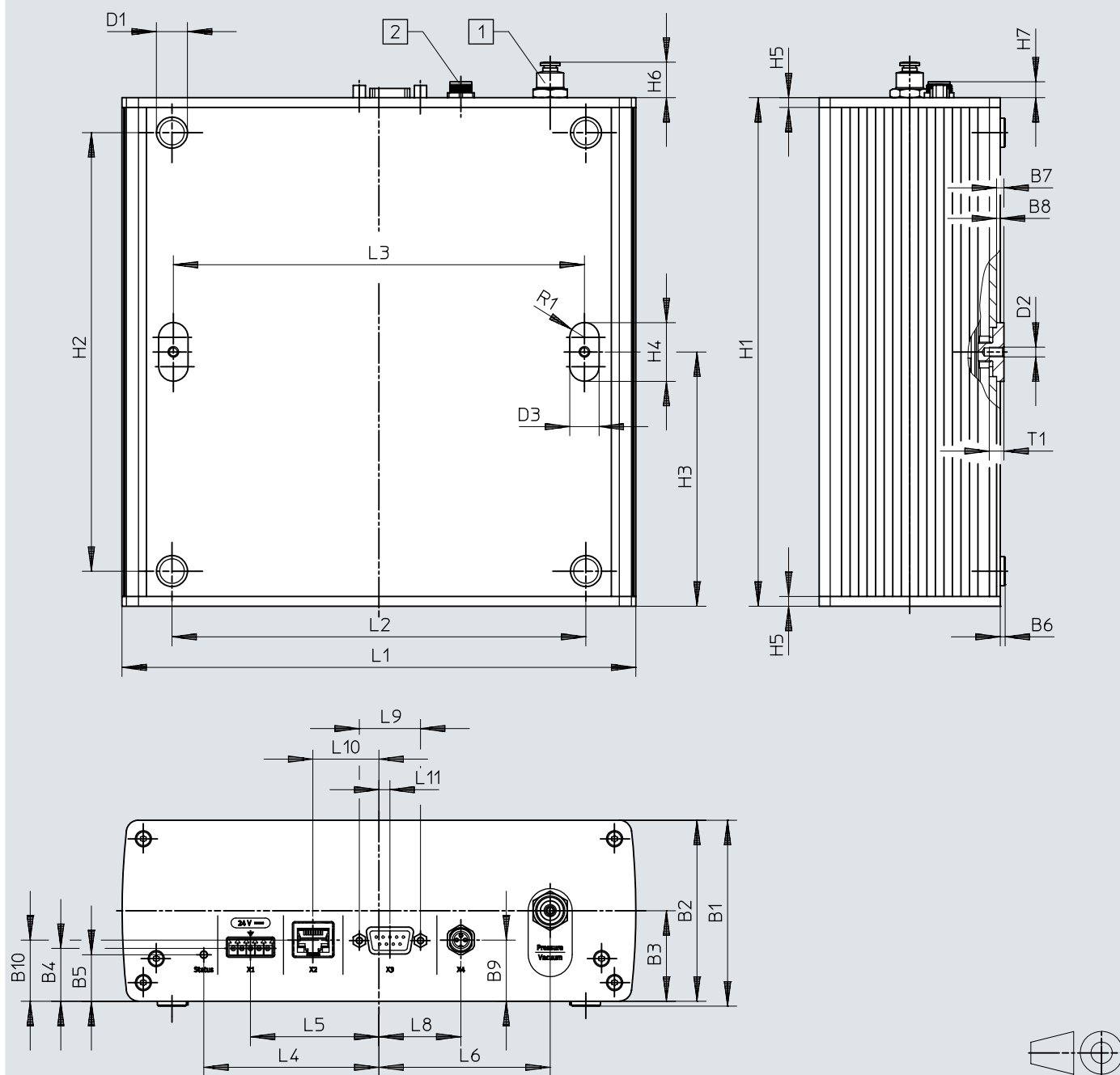
Dimensions – PGVA-1
