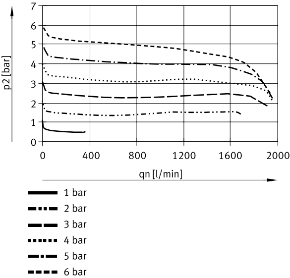
Standard flow rate qn as a function of output pressure p2 (p1 = 8 bar) – MS4-LR...-B
