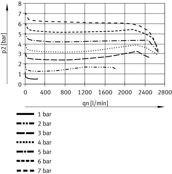
Standard flow rate qn as a function of output pressure p2 (p1 = 10 bar) – MS4-LR...-B
