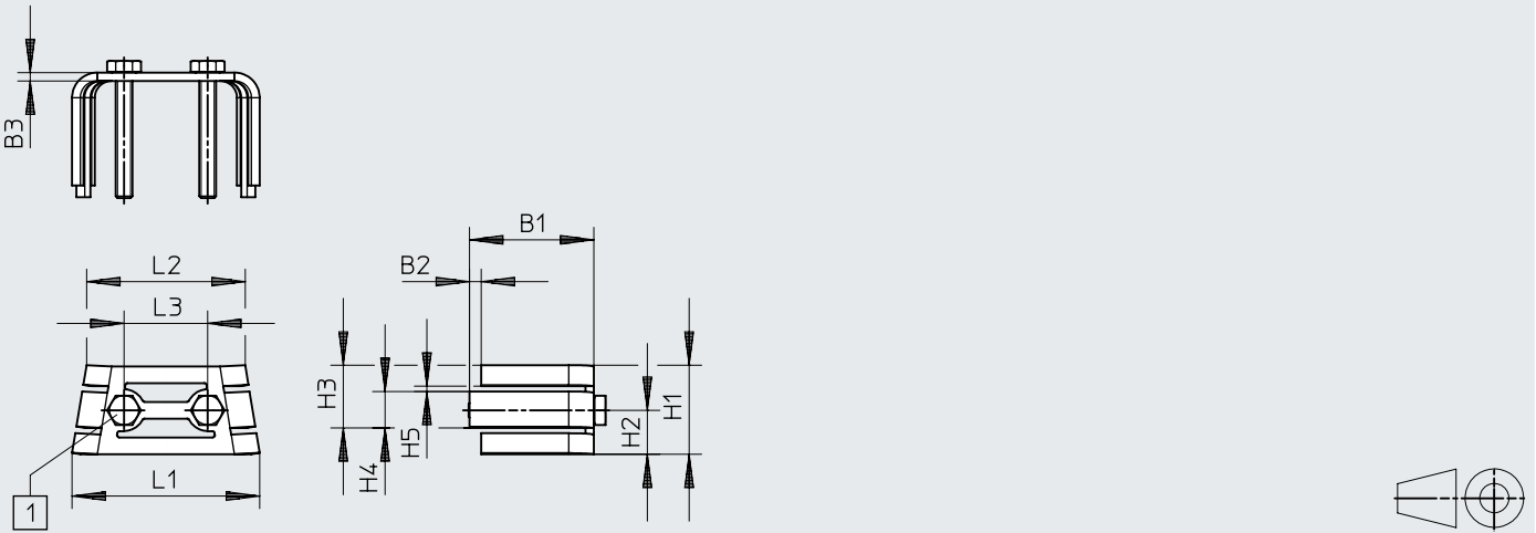
[1] Screws for size 120: ISO 4017-M4x30-A2-70
