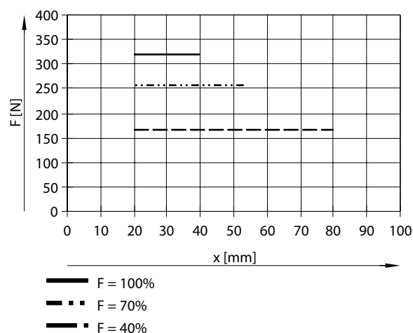
Total gripping force F as a function of lever arm x for HEPP-28
