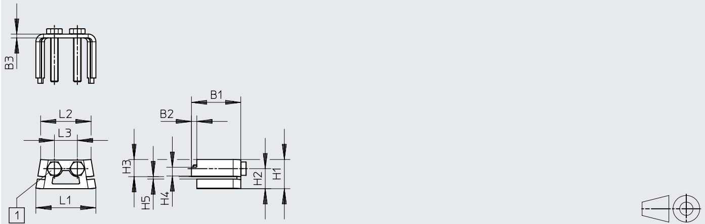
[1] Screws for size 60: ISO 4017-M3x22-A2-70; screws for size 80: ISO 4017-M4x25-A2-70
