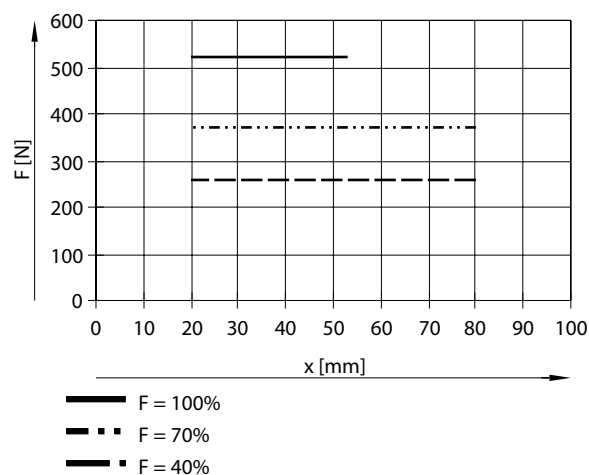
Total gripping force F as a function of lever arm x for HEPP-36
