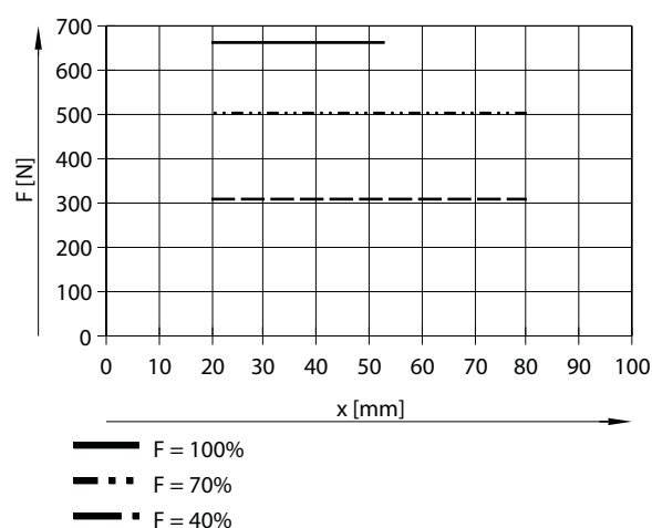
Total gripping force F as a function of lever arm x for HEPP-42
