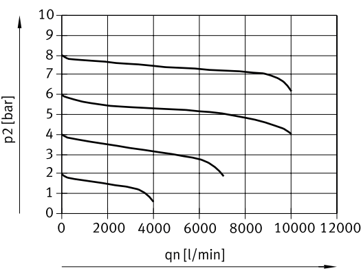
Standard flow rate qn as a function of output pressure p2 (FRC-1-D-MAXI)
