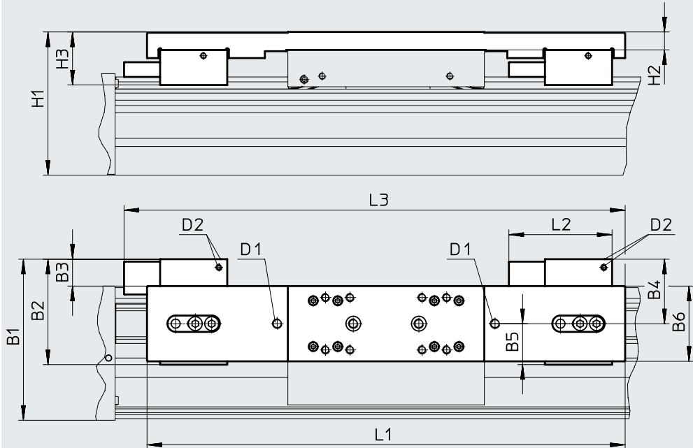
D2 Compressed air supply port
