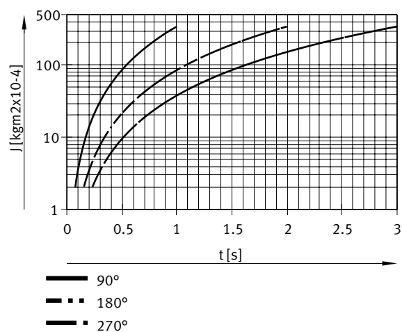
Mass moment of inertia J as a function of swivel time t – DRVS-40
