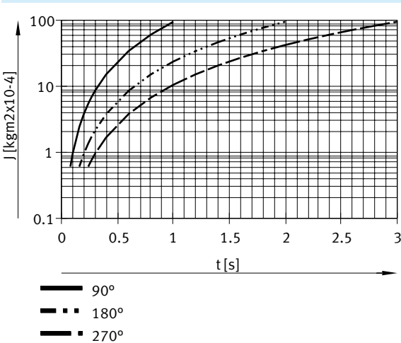
Mass moment of inertia J as a function of swivel time t – DRVS-16
