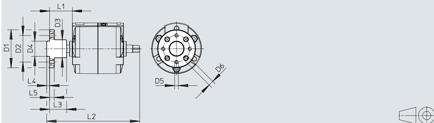
Dimensions – Push-on flange DARF-Q12-12 ... 16
