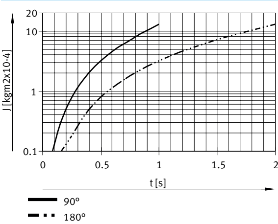
Mass moment of inertia J as a function of swivel time t – DRVS-8
