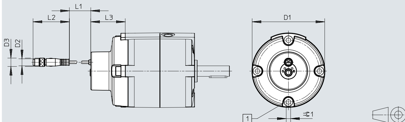
Dimensions – Position sensor SRBS-Q12-32 ... 40
