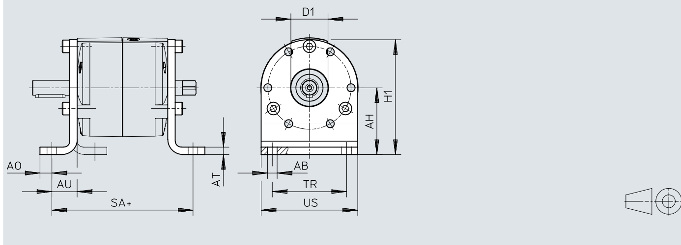
Dimensions – Foot mounting DAMH-Q12-12 ... 25
