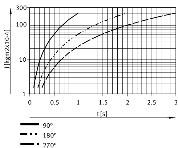
Mass moment of inertia J as a function of swivel time t – DRVS-32
