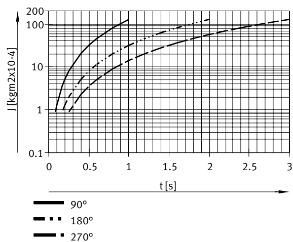
Mass moment of inertia J as a function of swivel time t – DRVS-25
