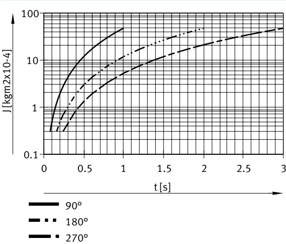
Mass moment of inertia J as a function of swivel time t – DRVS-12
