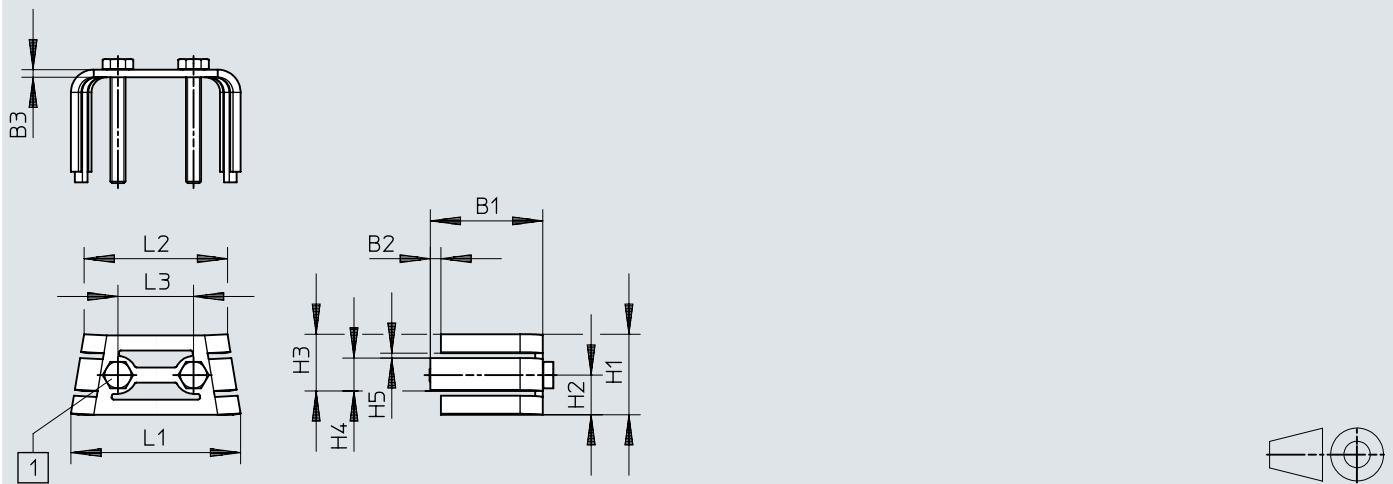
[1] DHAS-ME-H9-120: ISO 4017-M4x30-A2-70 screw
