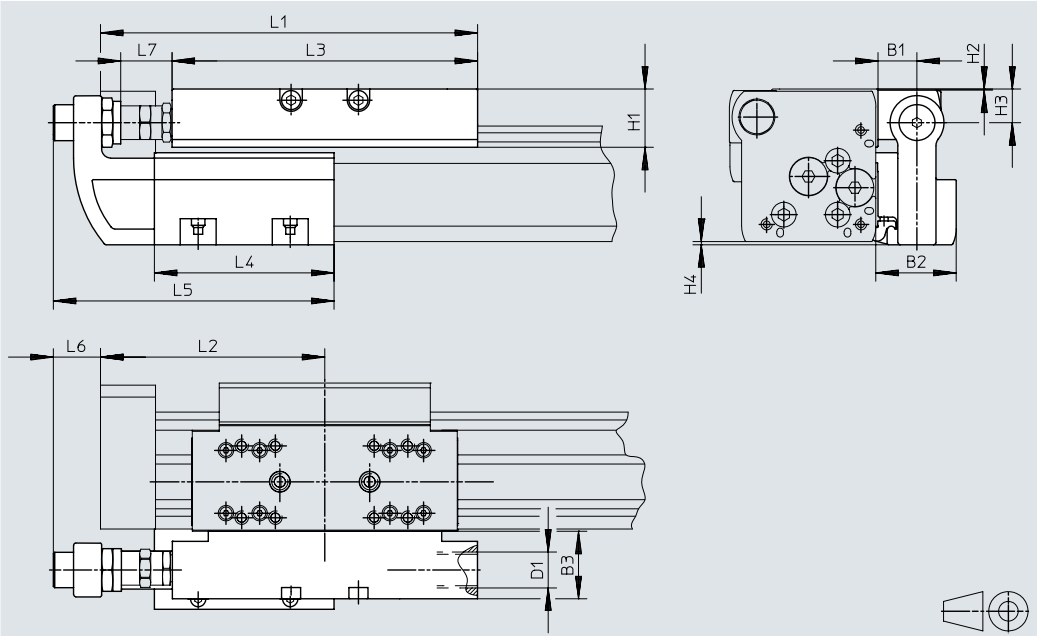
Shock absorber retainer DADP
