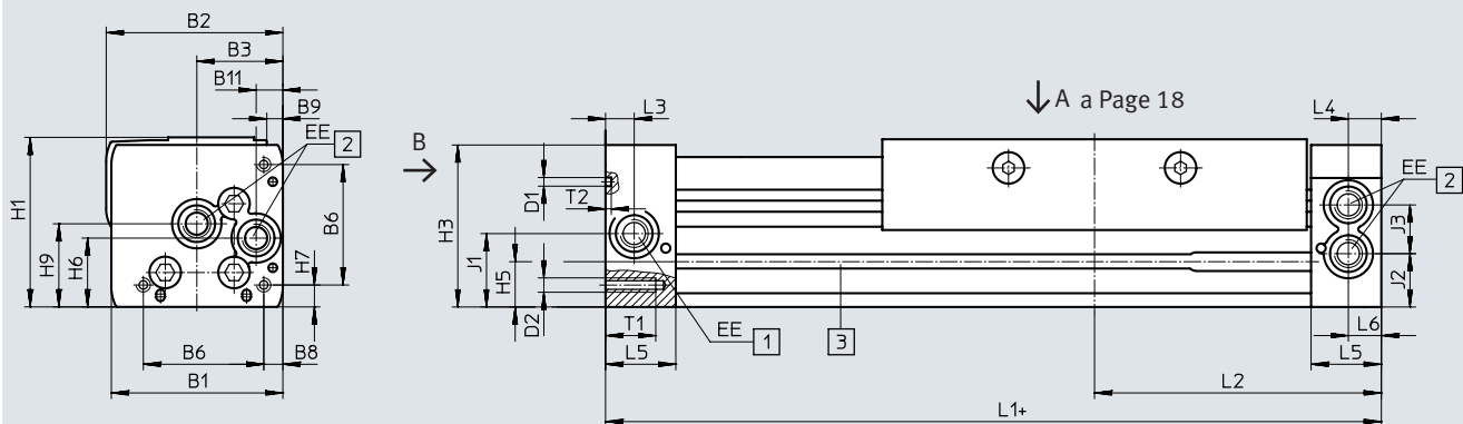
View B Ø 18
