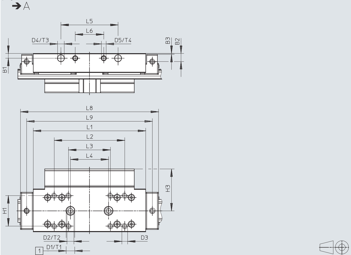
[1] Drilled hole for centring pin/sleeve
