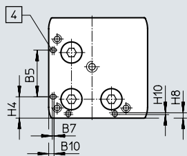
View B Ø 18
