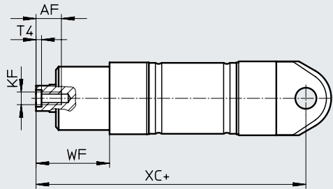
S2-K3 – Through piston rod, with female thread
