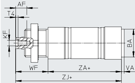
S2 – Through piston rod
